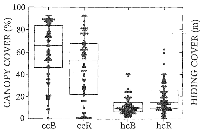
Figure 1. Canopy cover (in %) and hiding cover (in metres) for bed-sites (B) and random sites (R) showing plots of individual data and boxplots. Bed-sites had a denser canopy cover (ccB) and better hiding cover (hcB) than did random sites (ccR and hcR, respectively). One outlier is excluded from the figure for hcR. In the boxplots - the inside line gives the median, the upper boxline the upper quartile, the lower boxline the lower quartile. The horizontal lines above and below the box show the upper and lower fences, i.e. 1.5 times the distance between the median and the upper and lower quartiles (Wilkinson et al. 1992b).
